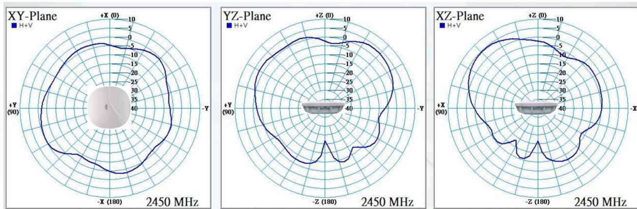
NWA 1050 – Scanning Radio - Normalized Radiation Pattern (2.4 GHz)
