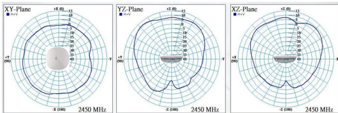
NWA 1050 – Client Serving - Normalized Radiation Pattern (2.4 GHz)
